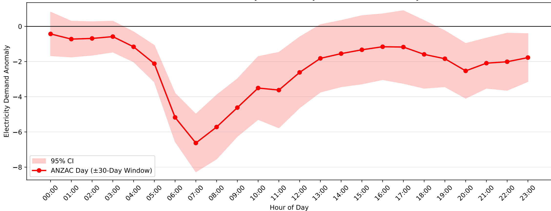
Meadowbank Demand Anomaly: ANZAC Day (2004-2017, \pm 30 -Day Window)
